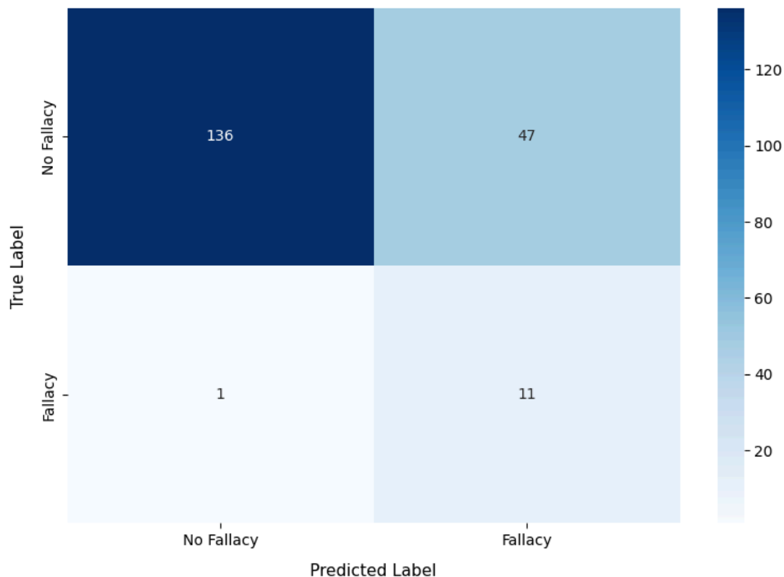
Confusion Matrix - gemma3:27b (zeroshot_no_extra, excluding timeouts)
